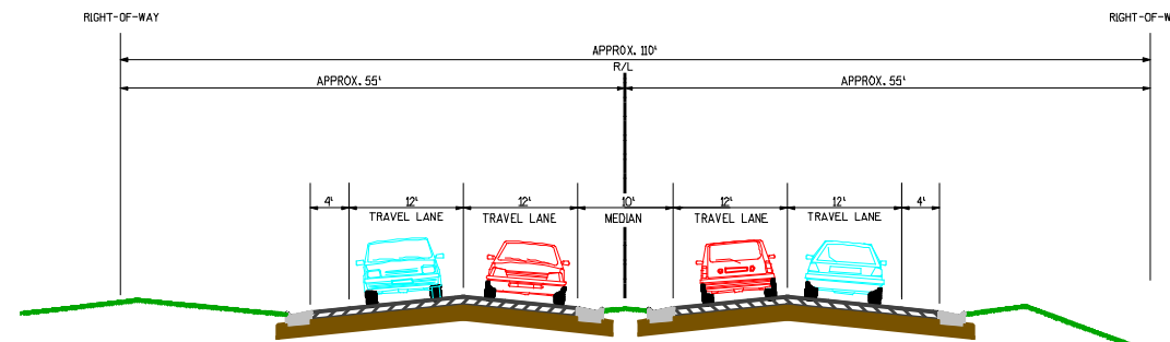
PROPOSED ROUNDABOUT ALTERNATIVE
