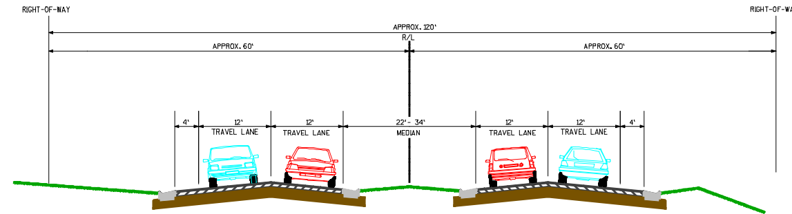
PROPOSED SIGNALIZED INTERSECTION ALTERNATIVE
