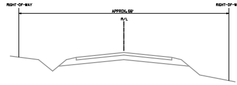
EXISTING SECTION
