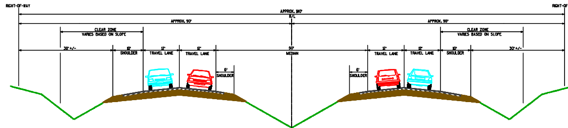
PROPOSED SECTION
