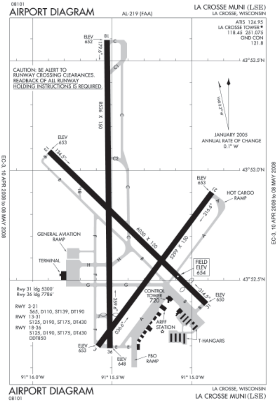
La Crosse Municipal Airport Diagram
